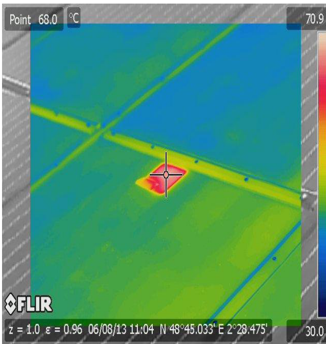
Figure (II.13) Imagerie infrarouge
