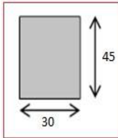
Figure 19II. Poutres PP (30x45 cm 2 )
