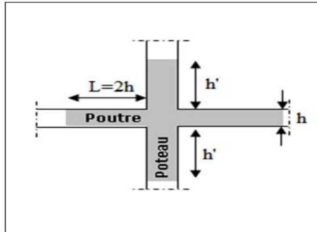
Figure 94.VI.:Zone nodale
