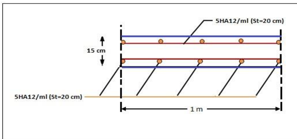
Figure 35.III.: Coupe A-A
