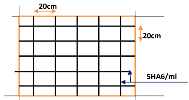
Figure 37.II. : Treillis soudés ( 20 \times 20 ) \text{cm}^2
