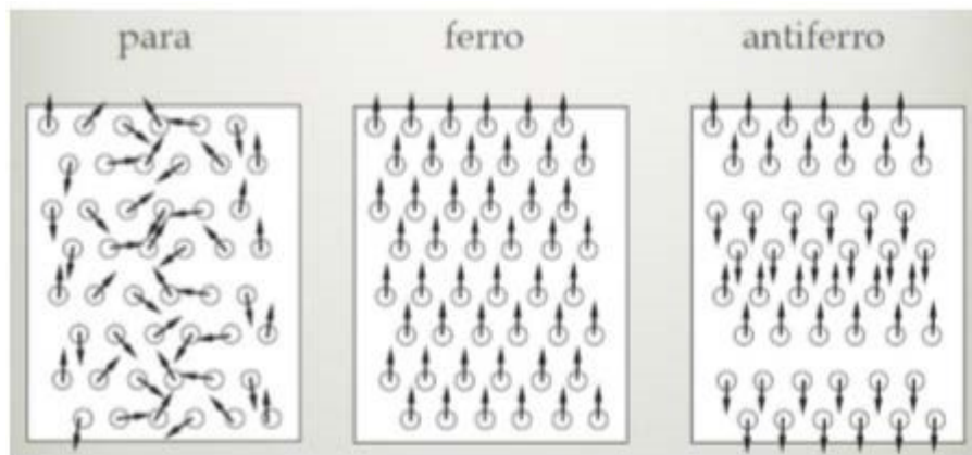
Figure I.4: Configurations magnétiques
