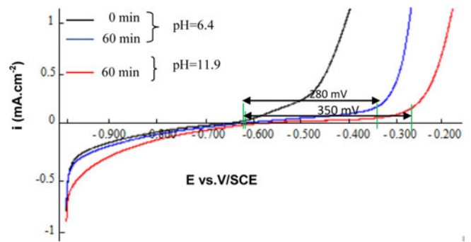
Fig. 6. Voltammograms of carbon steels exposed to the discharge for 60 min. Electrolyte 0.01 M NaNO 3 at different pH (6.5 and 11.9).
