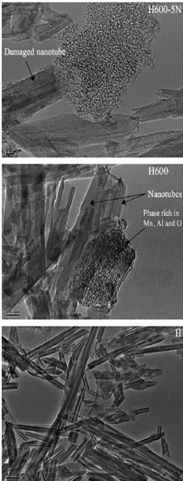
Figure.1 Transmission electron microscopy images of H, H600, and H600-5N.
