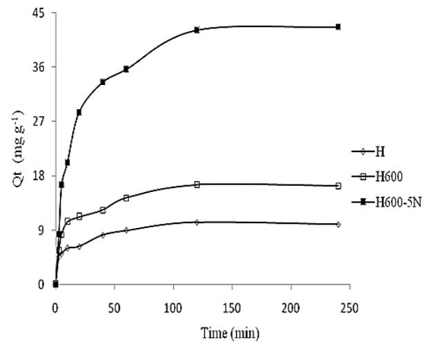
Figure.2 Effect of contact time on the uptake CR of H, H600 and H600-5N, at 55 °C
