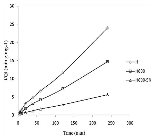
Figure.4 Pseudo second order kinetic for the adsorption of CR onto halloysitic solids
