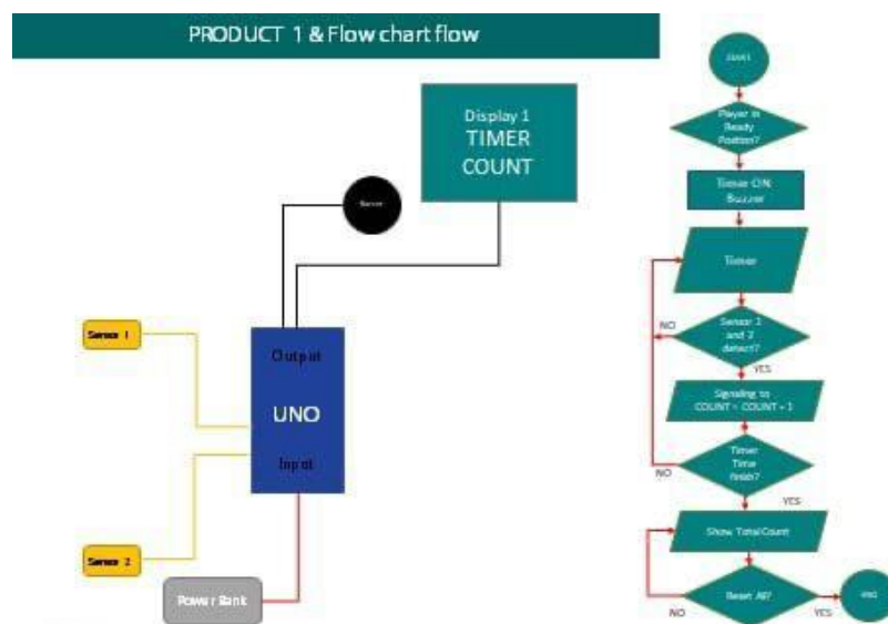
Figure 2 SATAS Flow Chart
